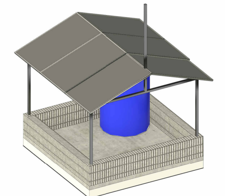
OG02 - Water Tower - Roof & Solar Construction
